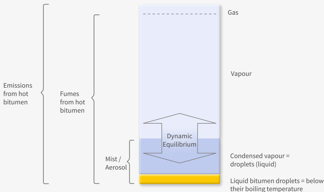
Figure 7. Schematic diagram of bitumen emissions
