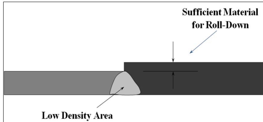
Figure 3. Longitudinal Cold Joint and Area of Low Density
