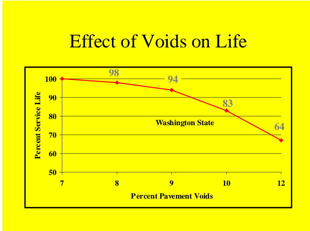
Figure 4. Low In-place Density versus Service Life (Washington Study, Ref 7)
