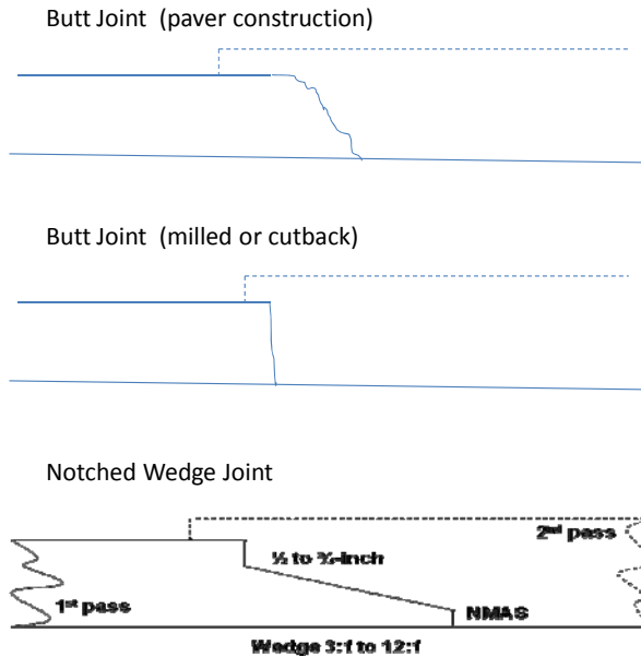
Figure 6. Butt Joint and Notch Wedge Joint
